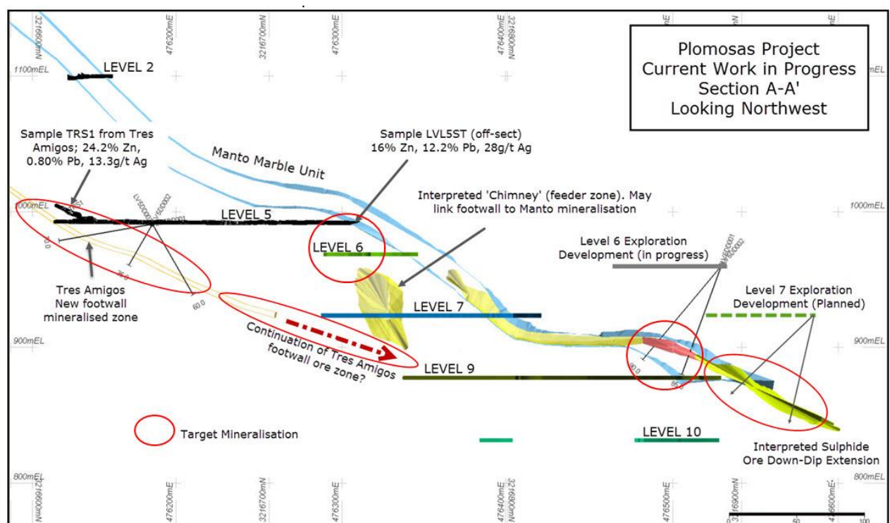
Figure 2. Plomosas Section A - A' (refer Figure 1) showing the current activities in the mine and spatial interpretations of various mineralised areas and exploration target zones
